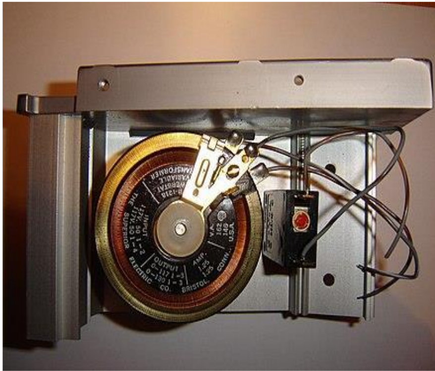
Auto-transformer with available secondary taps (60%,70% & 85 %)
